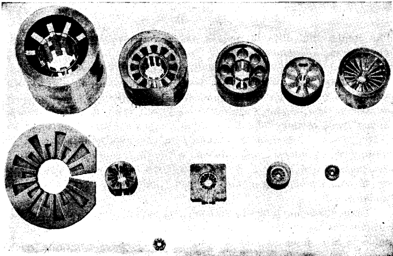
FIG. 1-27.—An array of anode blocks of different wavelength and power output. Top row: 10-cm, pulse power 2500 to 0.1 kw; second row: 3.2 cm, pulse power 600 to 0.025 kw; single block and insert 1.25 cm, 80 kw.
